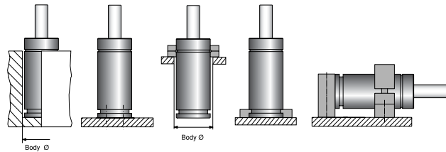
Drop - In MP Bottom Mount FC, FCS Top Mount LUG K, FFC Foot Mount S, HM Body Mount
